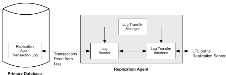
Figure 5-3: Sybase Replication Agent data flow
