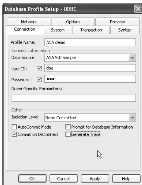
Figure 13-2: The Database Profile Setup dialog box
