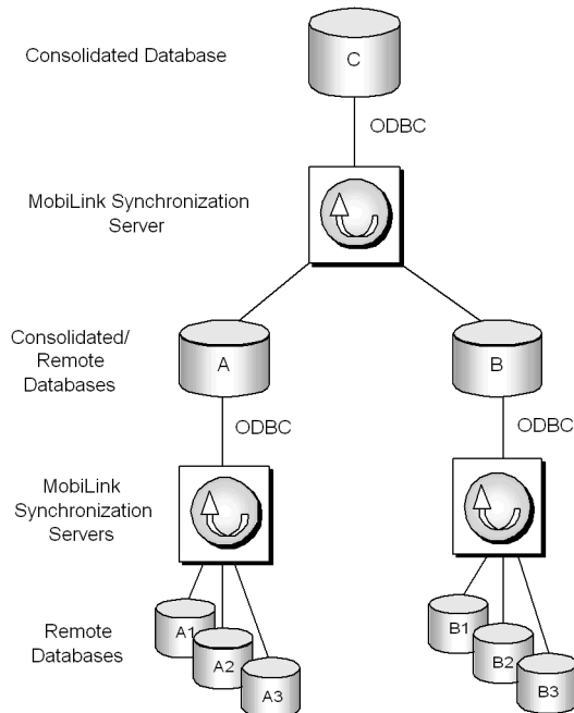
Figure 17-1: MobiLink hierarchy
