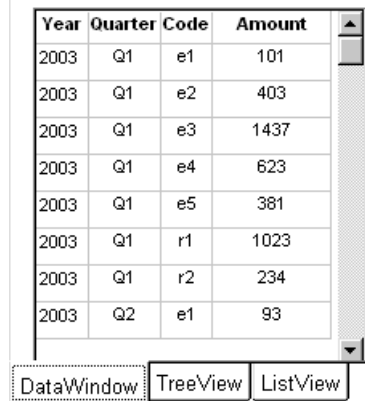
Figure 5-1: Tab control
