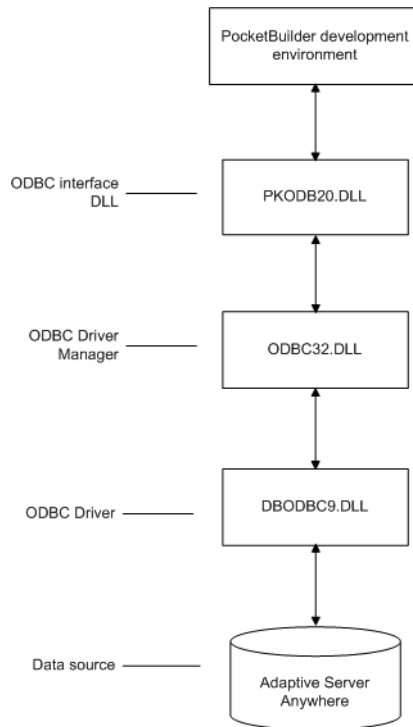
Figure 14-1: Components of an Adaptive Server Anywhere connection
