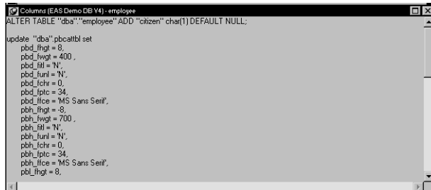
Figure 16-4: SQL syntax for pending changes to a table
