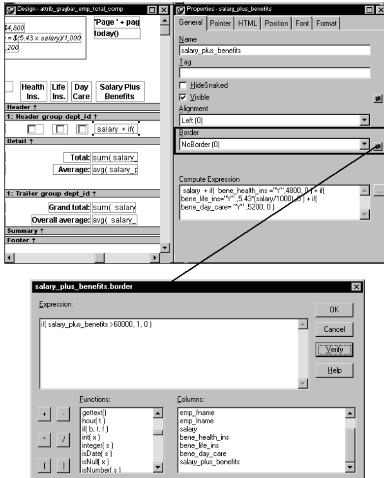
Figure 23-3: Setting a conditional expression for the Border property
