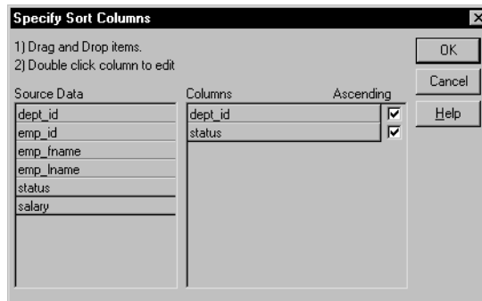
Figure 22-8: Sorting data by columns used to group data
