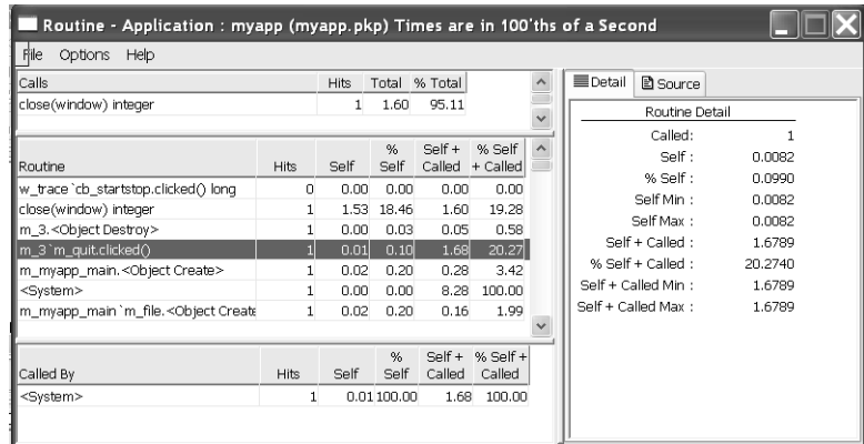
Figure 26-2: Profiling Routine View
