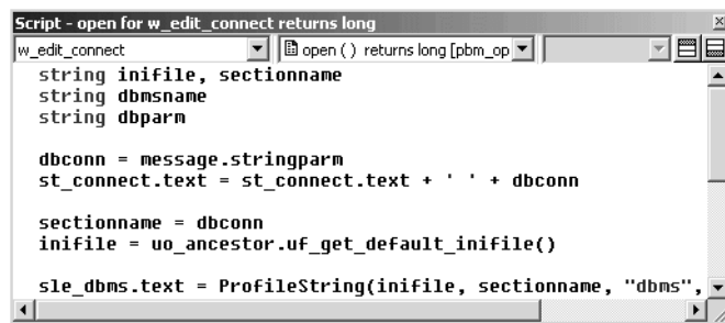
Figure 3-3: Script view for a window Open event
