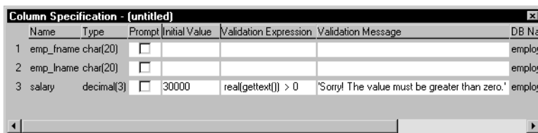
Figure 21-11: Specifying a validation rule in the DataWindow painter
