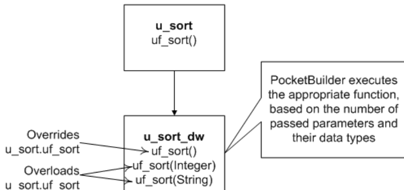
Figure 1-6: Function overloading
