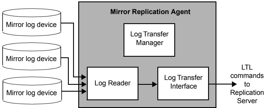
Figure 1-4: Mirror Replication Agent transaction data flow
