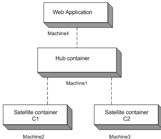
Figure 8-2: Sybase Search deployment architecture
