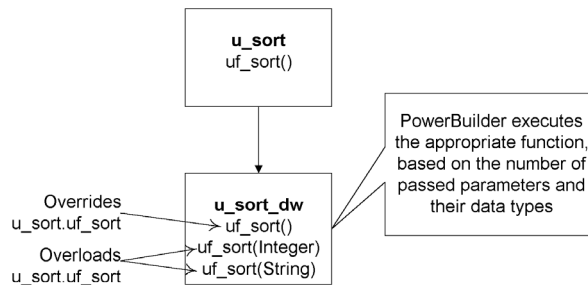
Figure 2-6: Function overloading
