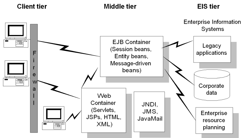
Figure 23-3: J2EE client, middle, and EIS tiers
