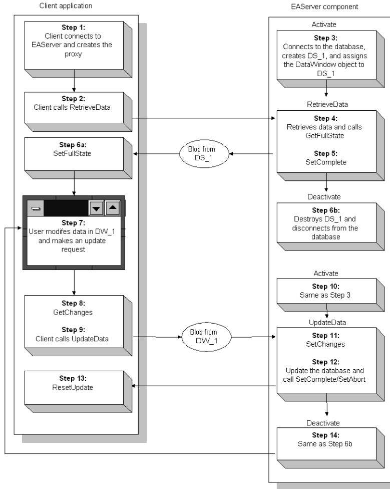
Figure 24-1: Update processing example
