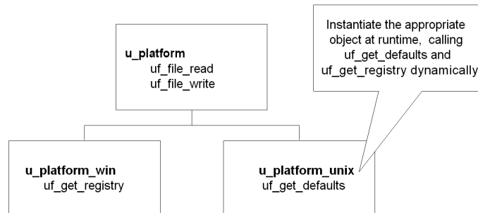
Figure 2-7: Dynamic lookup
