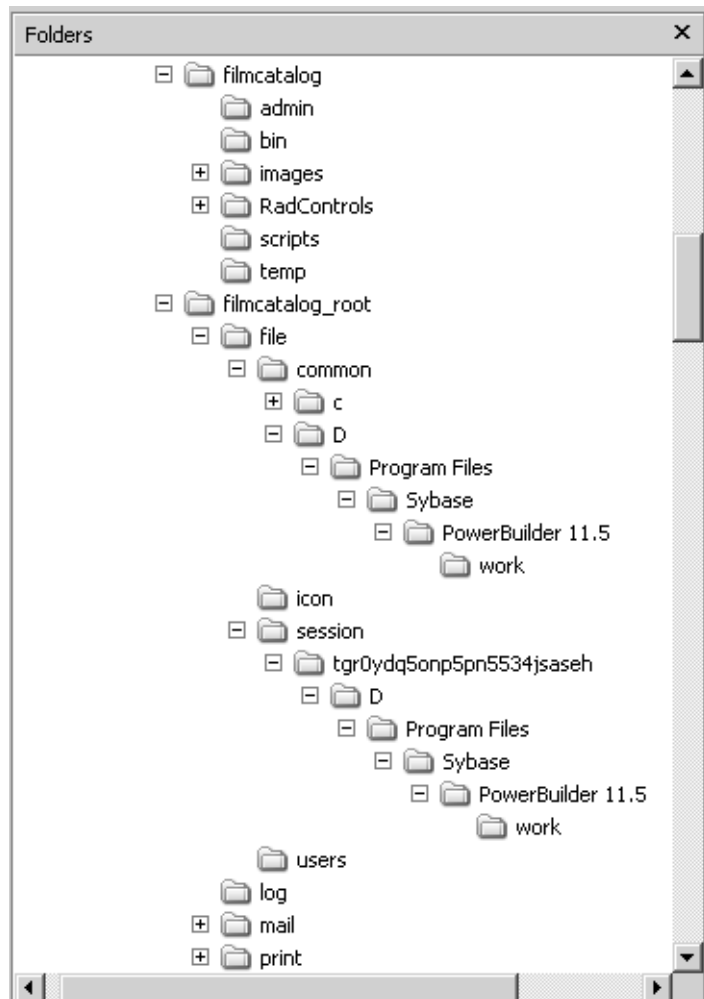
Figure 5-3: Virtual file system under the IIS root directory
